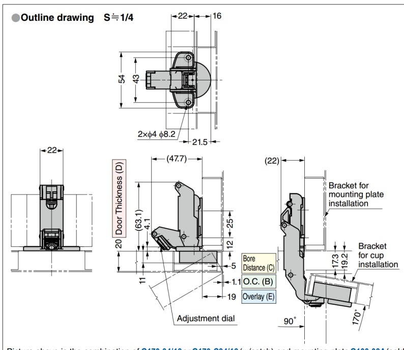
Picture above is the combination of G170-34/19 or G170-C34/19 (w/catch) and mounting plate G100-03A (sold separately).
