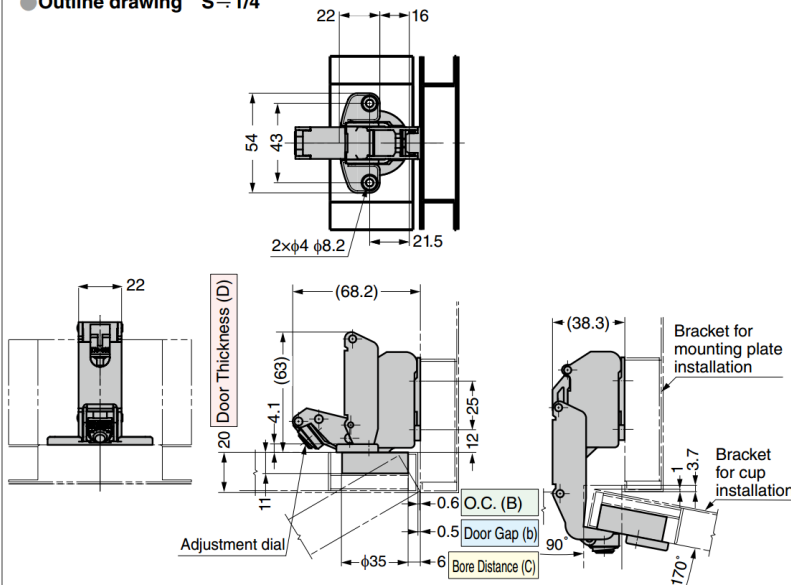
Picture above is the combination of G170-34/0 or G170-C34/0 (w/catch) and mounting plate G100-03A (sold separately).
